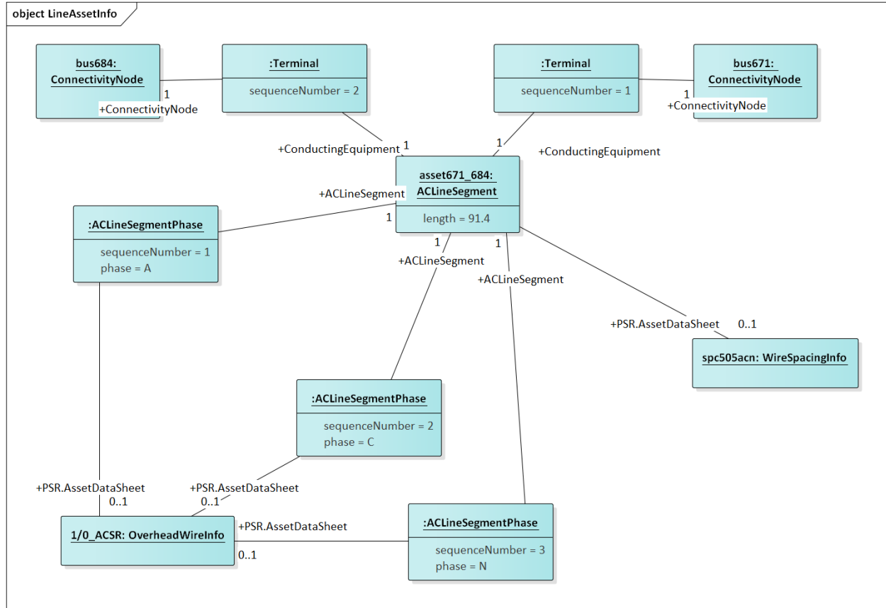
Figure 32: The two-phase ACLineSegment impedance defined by sharing wire and spacing data from a catalog. Each ACLineSegmentPhase links to an OverheadWireInfo instance via the AssetDataSheet association. If the neutral (N) is present, we have to specify its wire information for a correct impedance calculation. In this case, ACN all use the same wire type, but they can be different, especially for the neutral. Similarly, the WireSpacingInfo associates to the ACLineSegment itself via a AssetDataSheet association.
